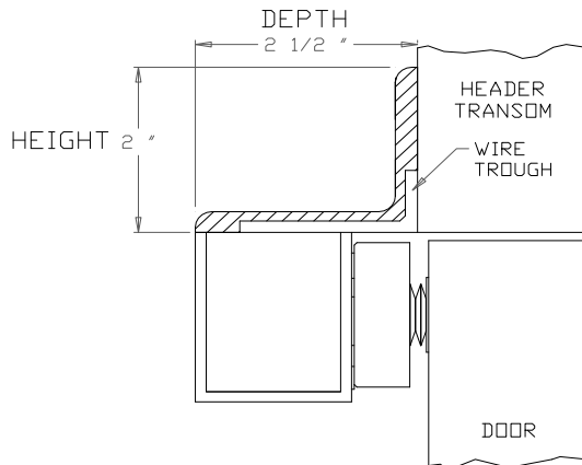
1194 ANGLE BRACKET
