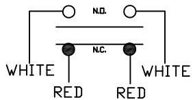
PNEUMATIC DELAY -P23DA
