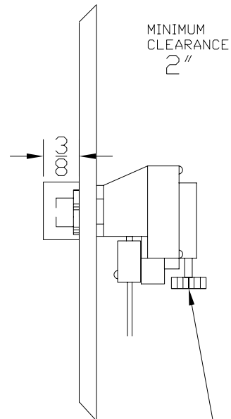
PNEUMATIC SWITCH 2-60 SECOND ADJUSTMENT KNOB
