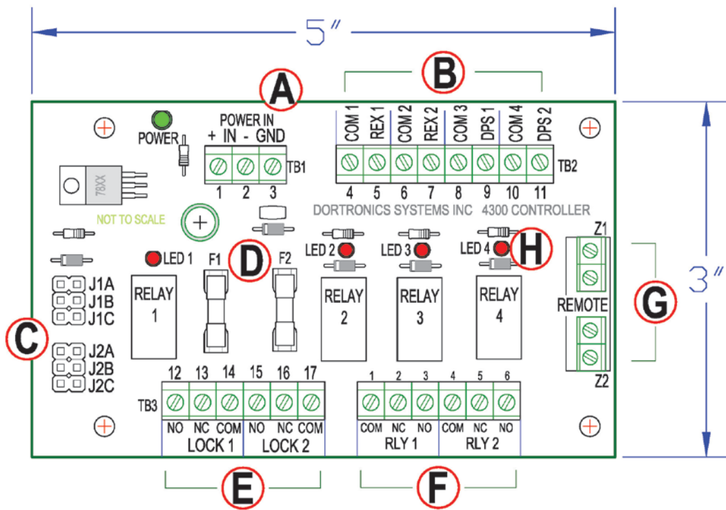
FIG. 1 CONTROLLER DIAGRAM
