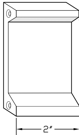
PART# - 3382 2" BRACKET
