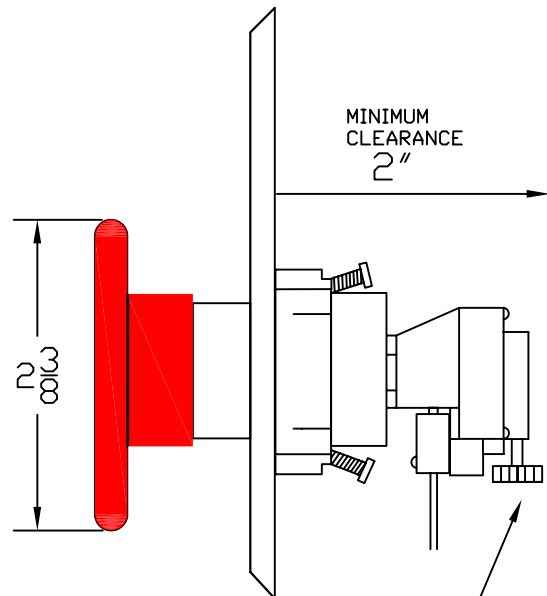
PNEUMATIC SWITCH 2-60 SECOND ADJUSTMENT KNOB
